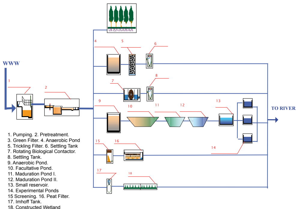
Figure 2. Flow diagram of the Technological Transfer Centre, Morocco. (Fahd et al. , 2007).
